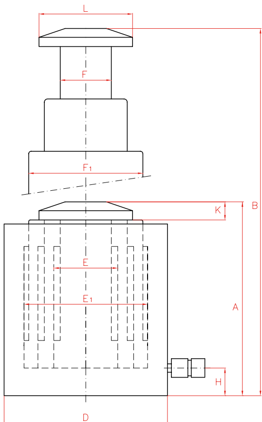
Telescopic Aluminium Cylinders, DLA.
